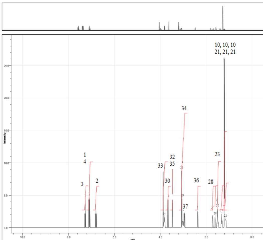
Figure 47: Better resolution of ^1\text{H-NMR} spectrum of (AZ-4) by Marvin Sketch.
